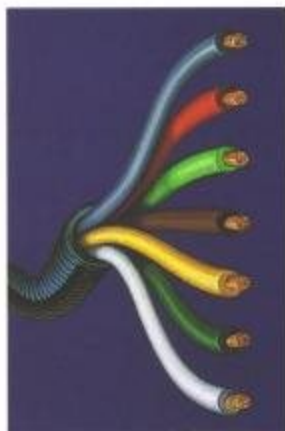
▲ An optional 5-wire wiring harness is used with trailers up to 2000 lbs. gross weight, and a 7-wire for larger trailers. Harnesses tie into the vehicle's electrical system to provide electricity for your trailer's lights, electric brakes or battery charging. This color code for Chevy trucks should be used when installing trailer wiring harnesses:
