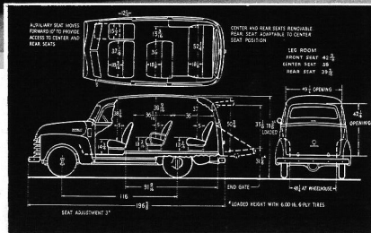
MODEL 3116 CARRYALL SUBURBAN 116-INCH WHEELBASE, MAXIMUM G.V.W. 4600 LB.
