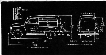
MODEL 3107 CANOPY EXPRESS 116-INCH WHEELBASE, MAXIMUM G.V.W. 4600 LB.
