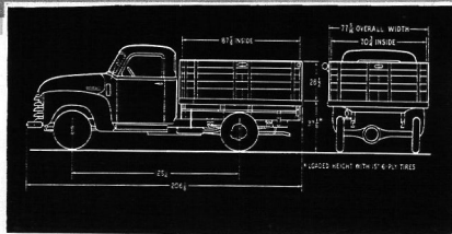
MODEL 3609 *DE LUXE STAKE 128 \frac{1}{2} -INCH WHEELBASE, MAXIMUM G.V.W. 5800 LB.
