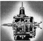
Four-Speed Transmission. Synchroneshifting into second, third, and high gears. May be had instead of three-speed unit in all models except Sedan Delivery.
