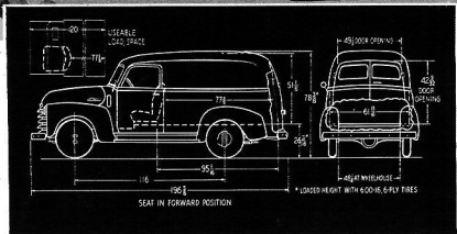
MODEL 3105 *DE LUXE PANEL 116-INCH WHEELBASE, MAXIMUM G.V.W. 4600 LB.
