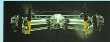
FULLY INDEPENDENT REAR SUSPENSION A unique 5-link independent rear suspension with a transverse monoleaf spring helps put power to the pavement.
