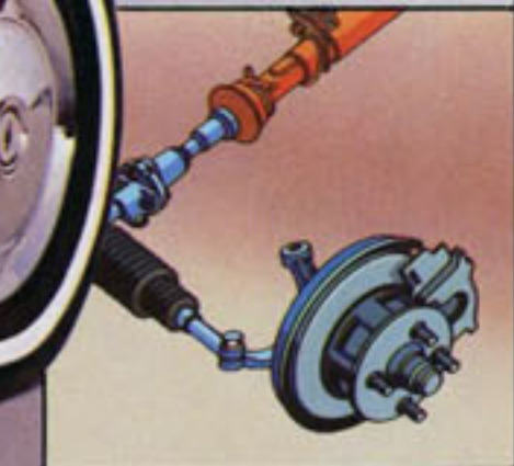
RACK-AND-PINION STEERING.
