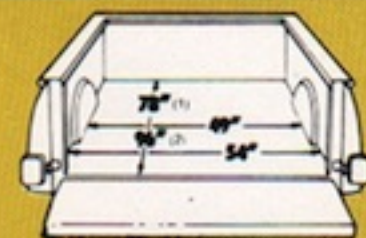
Two Utiline bodies (1) 6½-foot box, 47.25-cubic foot capacity (2) 8-foot box, 58.50-cubic foot capacity
